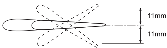
Aileron Control
