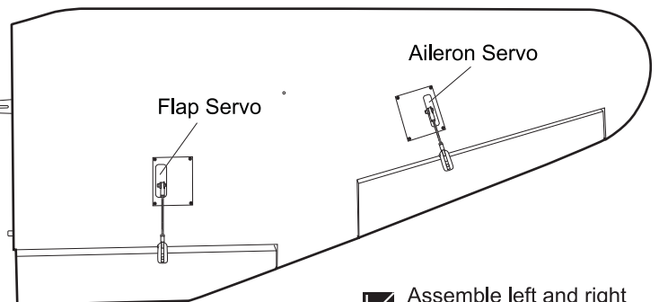
< Left Wing >
