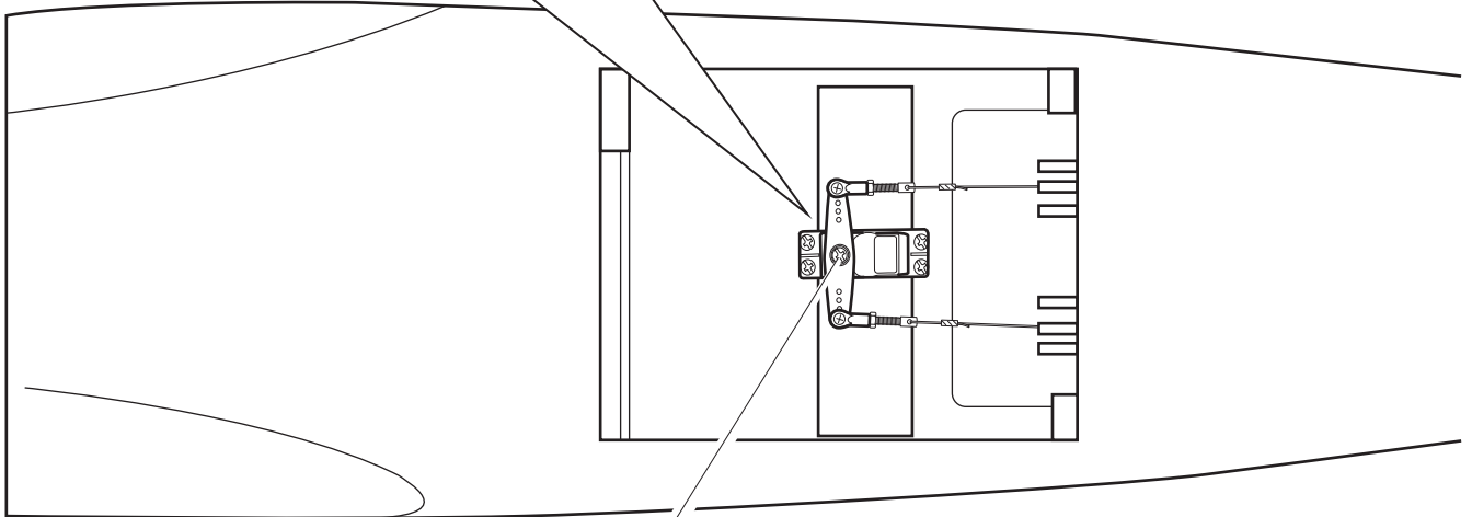
Rudder servo
