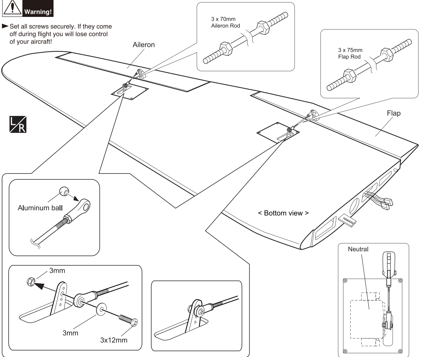
< Right Wing >
