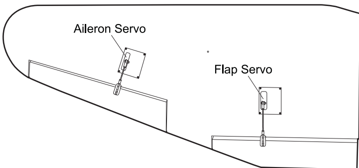
< Right Wing >
