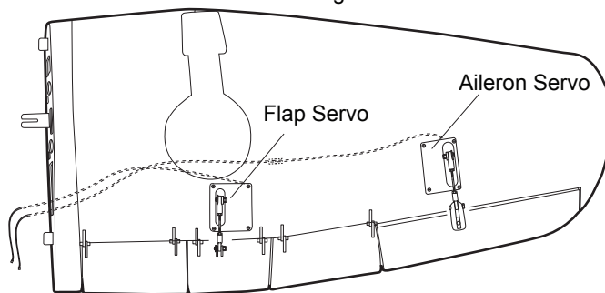
< Left Wing >
