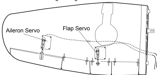
< Right Wing >
