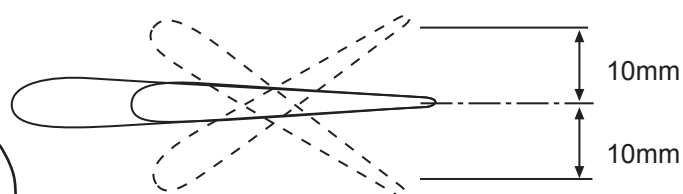
Aileron Control
