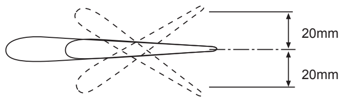
Rudder Control
