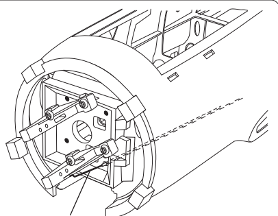
Throttle Rod
