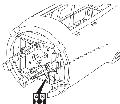
Throttle Rod
